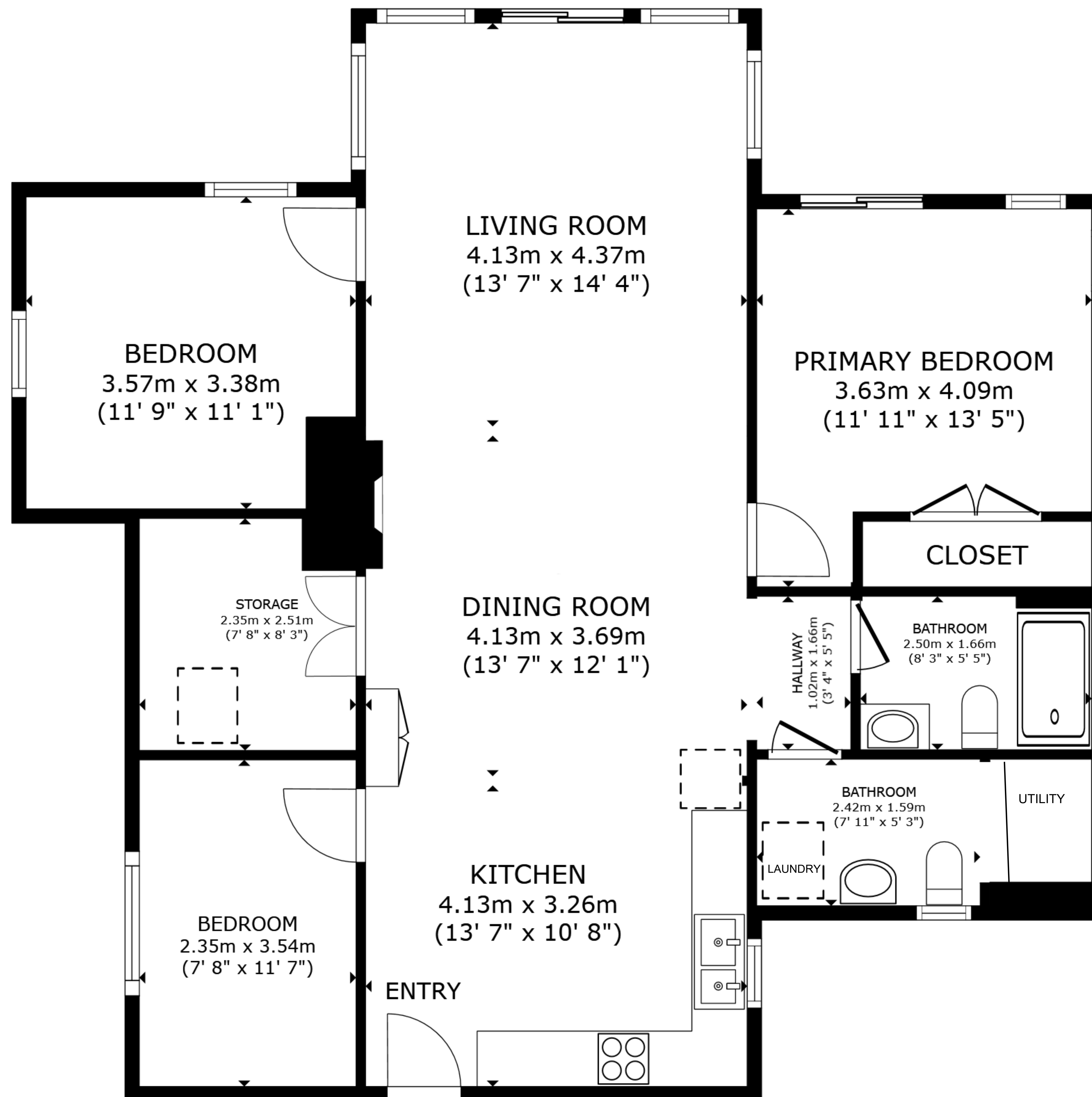
FLOOR PLAN
